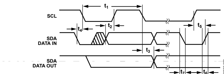
Figure 2 I 2 C Timing Diagram
