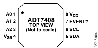
Figure 4. Pin Configuration
