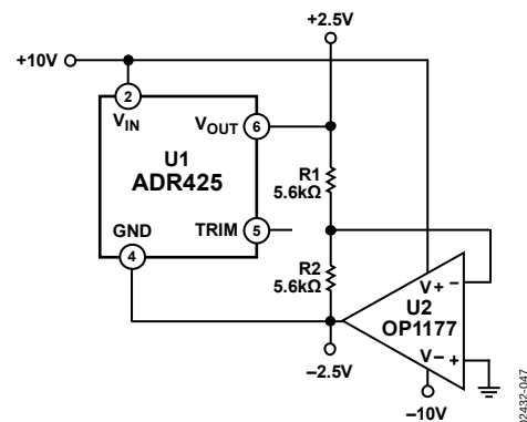
Figure 46. +2.5 V and -2.5 V Reference Using ADR425
