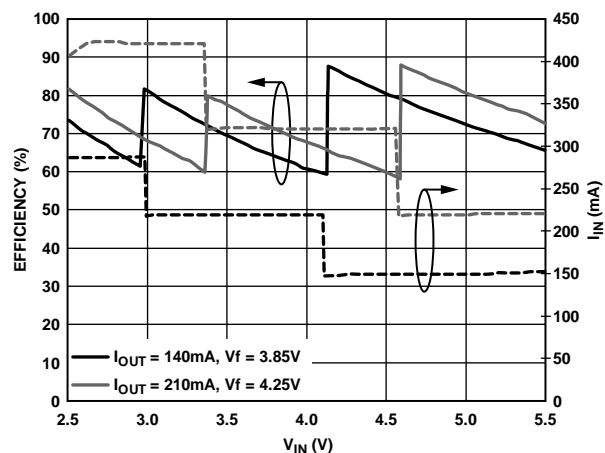
Figure 20. Typical Efficiency (High V_f Diode)
