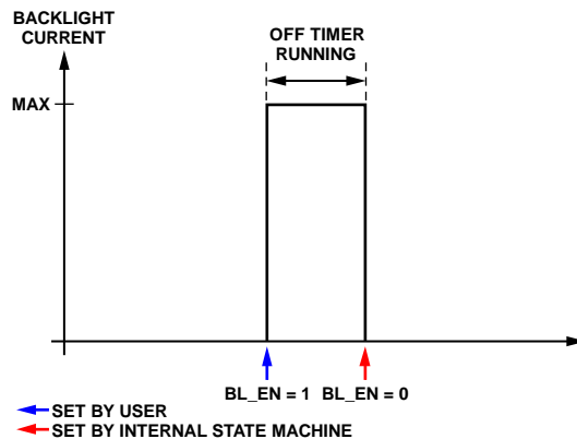
Figure 34. Off Timer
