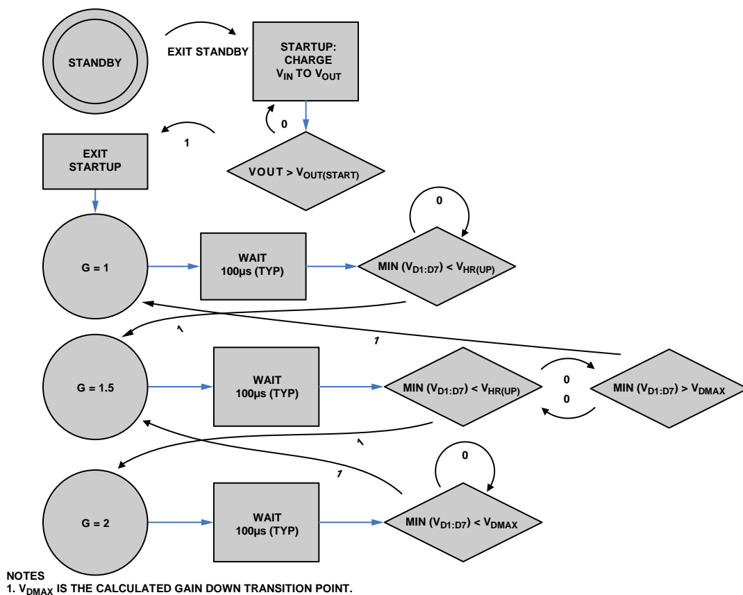
Figure 26. State Diagram for Automatic Gain Selection Rev. A | Page 12 of 40
