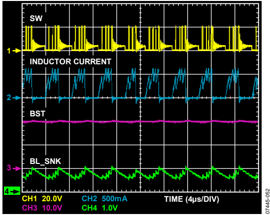
Figure 9. Boost Operation (Backlight = 30 mA)
