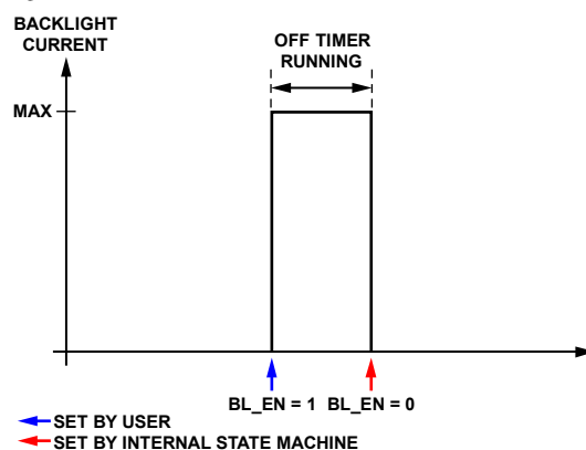
Figure 20. Off Timer
