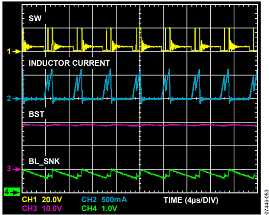
Figure 10. Boost Operation (Backlight = 15 mA)
