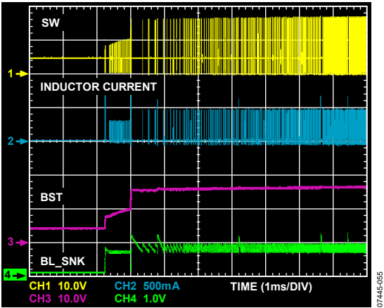
Figure 12. Boost Startup
