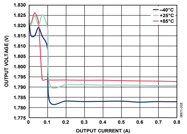
Figure 8. Buck Load Regulation Across Temperature, VOUT1 = 1.8 V, Auto Mode
