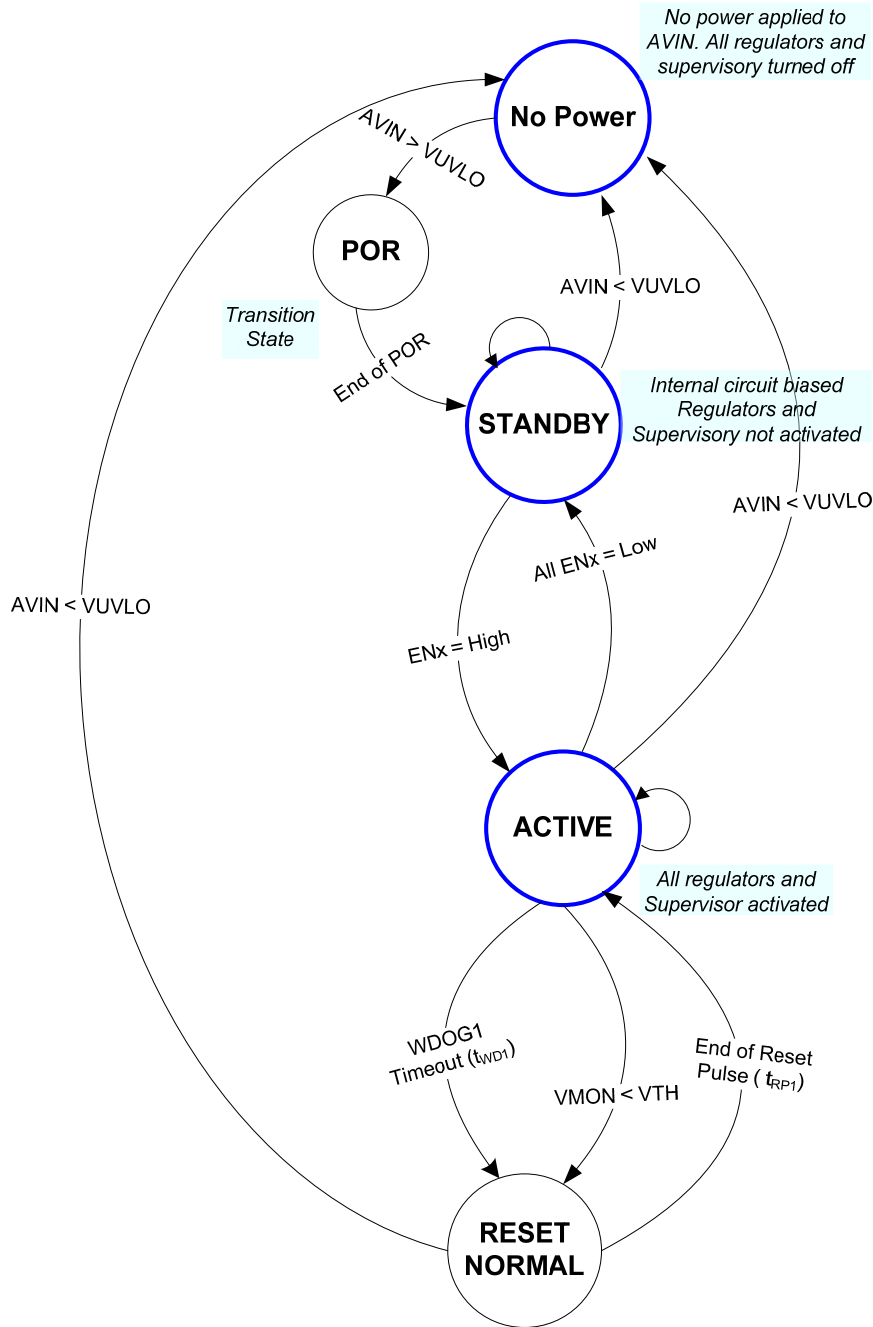
Figure 62. ADP5041 State Flow
