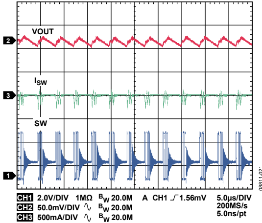
Figure 21. Typical Waveforms, V_{OUT1} = 1.8\text{ V} , I_{OUT1} = 30\text{ mA} , Auto Mode
