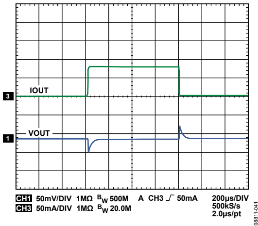
Figure 41. LDO1 Response to Load Transient, IOUT2 from 1 mA to 80 mA, VOUT2 = 1.5 V
