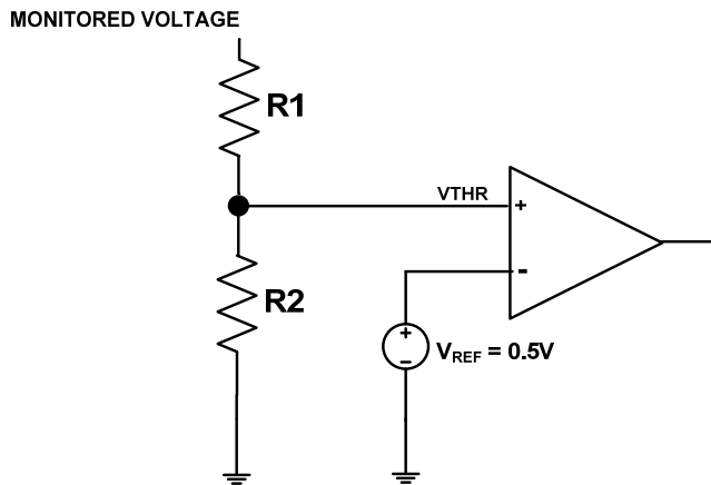
Figure 60. External Reset Threshold Programming.
