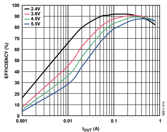
Figure 14. Buck Efficiency vs. Load Current, Across Input Voltage, V_{OUT1} = 1.8\text{ V} , PWM Mode
