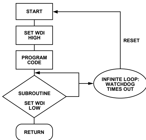
Figure 67. Watchdog Flow Diagram
