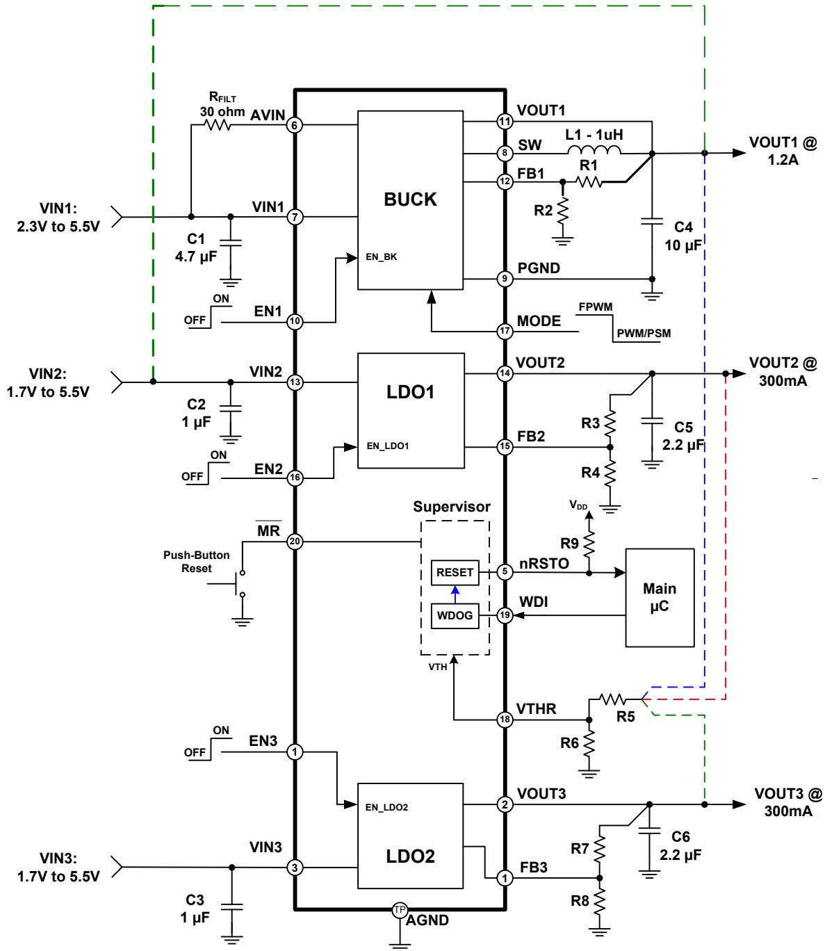
Figure 69. Application Diagram
