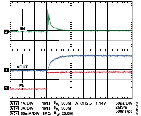
Figure 30. LDO1 Startup, VOUT2=1.5 V, IOUT2 = 5 mA
