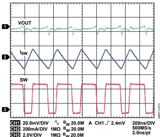
Figure 23. Typical Waveforms, V_{OUT1} = 3.3\text{ V} , I_{OUT1} = 30\text{ mA} , PWM Mode
