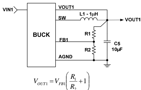
Figure 57 Buck External Output Voltage Setting
