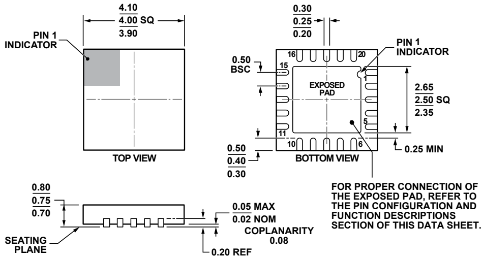
Figure 70. 20-Lead Lead Frame Chip Scale Package [LFCSP_WQ] 4 mm × 4 mm Body, Very Very Thin Quad (CP-20-10) Dimensions shown in millimeters
