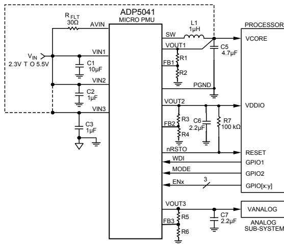
Figure 64. Processor System Power Management with PSM/PWM Control
