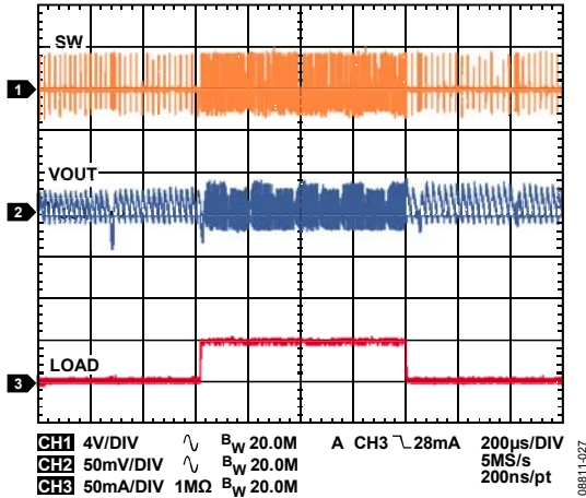
Figure 27. Buck Response to Load Transient, IOUT1 from 1 mA to 50 mA, VOUT1 = 1.8 V, Auto Mode
