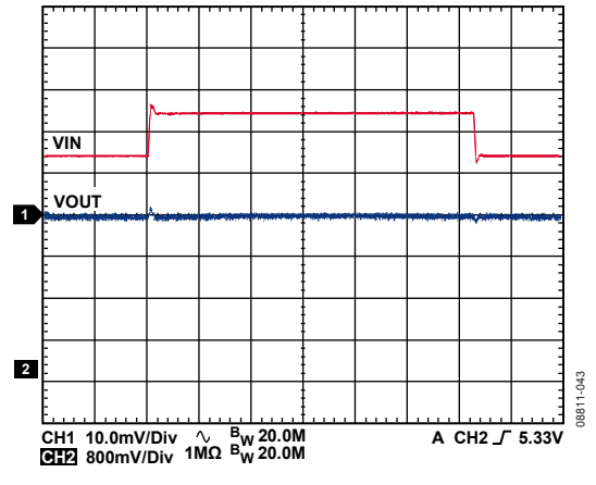
Figure 43. LDO1 Line Transient VIN2 = 4.5 V to 5.5 V, VOUT2 = 1.5 V
