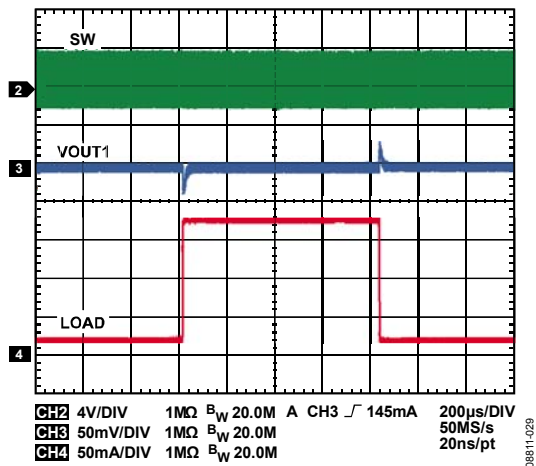
Figure 29. Buck Response to Load Transient, IOUT1 from 20 mA to 180 mA, VOUT1 = 1.8 V, PWM Mode
