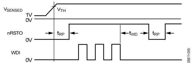
Figure 61. Watchdog Timing Diagram
