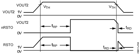
Figure 59. Reset Timing Diagram
