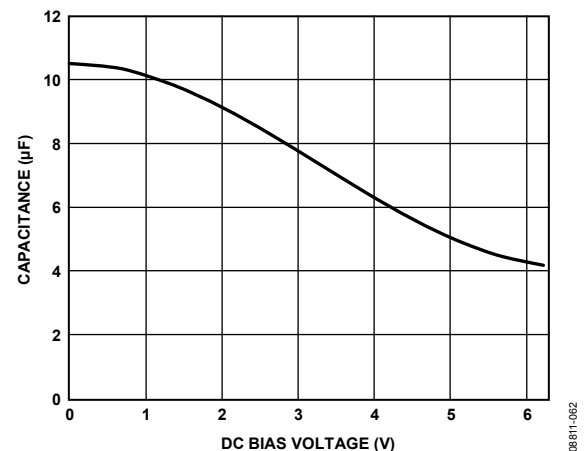
Figure 63. Typical Capacitor Performance
