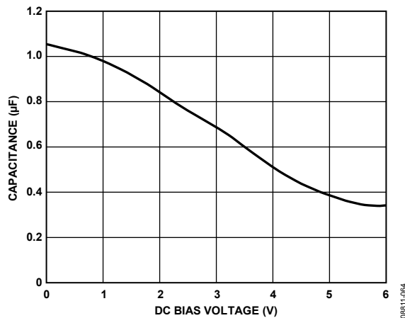
Figure 65. Capacitance vs. Voltage Characteristic
