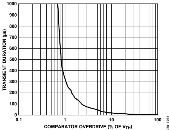
Figure 66. Maximum V_{TH} Transient Duration vs. Reset Threshold Overdrive
