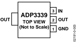
NOTE: PIN 2 AND TAB ARE INTERNALLY CONNECTED Figure 3. 3-Lead SOT-223 Pin Configuration
