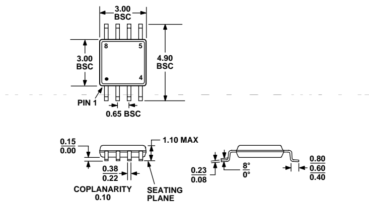
Figure 27. 8-Lead Mini Small Outline Package [MSOP] (RM-8)
