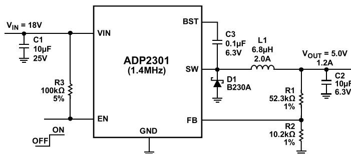
图56. ADP2301—1.4MHz典型应用, V_{IN}=18V , V_{OUT}=5V/1.2A , 带外部使能
