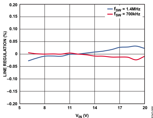
图13. 电压调整率, V_{OUT} = 3.3V , I_{OUT} = 500mA
