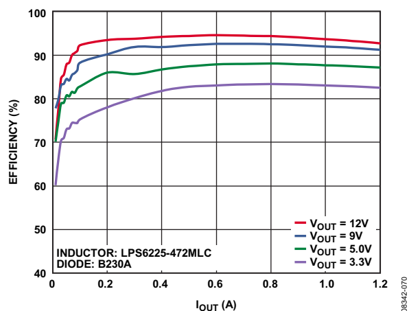
图4. 功效曲线, V_{IN} = 18\text{ V} , f_{SW} = 1.4\text{ MHz}
