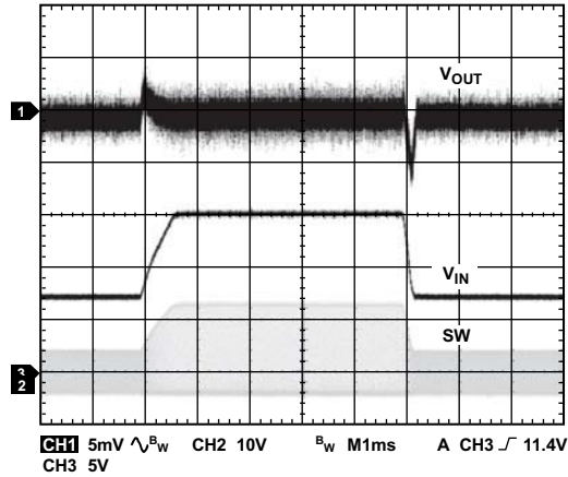
图34. ADP2301线性瞬态响应, 7V 至 15V , V_{OUT} = 3.3V , I_{OUT} = 1.2A , f_{SW} = 1.4MHz
