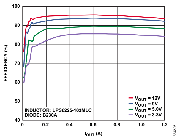
图5. 功效曲线, V_{IN} = 18\text{ V} , f_{SW} = 700\text{ kHz}
