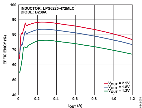
图8. 功效曲线, V_{IN} = 5.0\text{ V} , f_{SW} = 1.4\text{ MHz}
