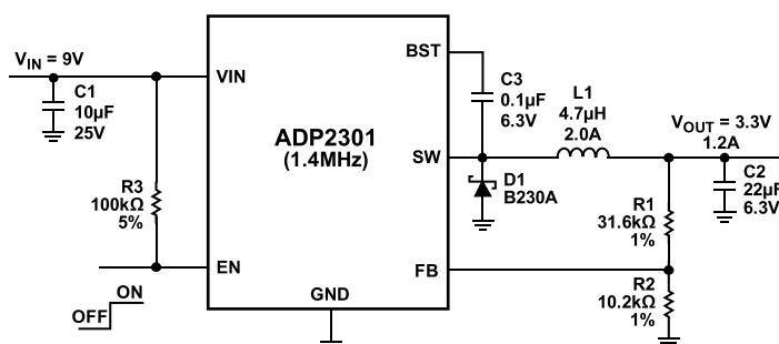
图57. ADP2301—1.4MHz典型应用, V_{IN}=9V , V_{OUT}=3.3V/1.2A , 带外部使能
