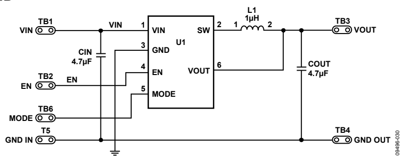
Figure 36. Evaluation Board Schematic
