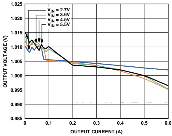
Figure 10. Load Regulation, V_{OUT} = 1.0\text{ V}
