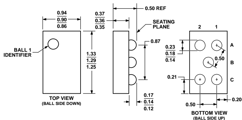
Figure 33. 5-Ball Wafer Level Chip Scale Package [WLCSP] (CB-5-1) Dimensions shown in millimeters
