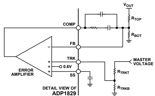
Figure 30. Voltage Tracking
