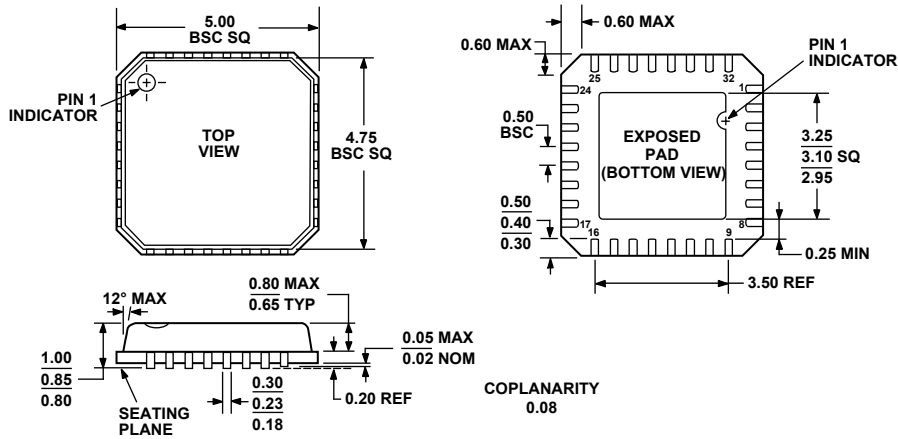
COMPLIANT TO JEDEC STANDARDS MO-220-VHHD-2 Figure 36. 32-Lead Lead Frame Chip Scale Package [LFCSP_VQ] 5 mm x 5 mm Body, Very Thin Quad (CP-32-2) Dimensions shown in millimeters
