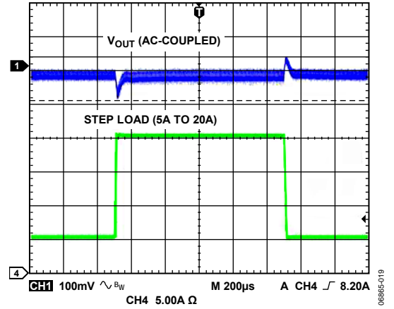
Figure 19. Load Transient Response of Figure 1, 5 A to 20 A, V_{IN} = 12 V
