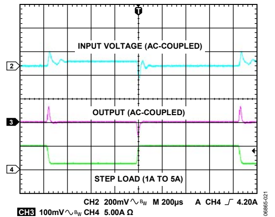
Figure 21. Load Transient Response of Figure 54, 1 A to 5 A, V_{IN} = 12 V
