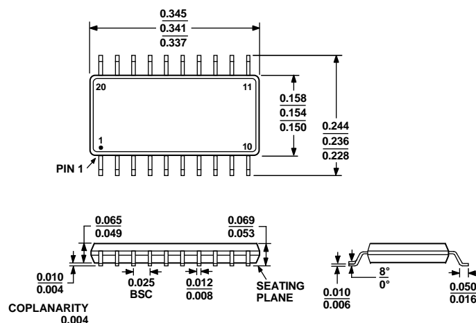
COMPLIANT TO JEDEC STANDARDS MO-137-AD Figure 57. 20-Lead Shrink Small Outline Package [QSOP] 150 mil Body (RQ-20) Dimensions shown in inches
