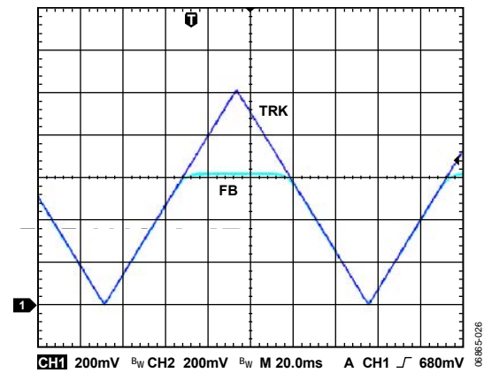
Figure 26. Tracking, TRK from 0 V to 1 V
