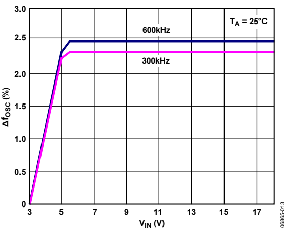
Figure 13. \Delta f_{OSC} vs. V_{IN} , Referenced at V_{IN} = 3 V
