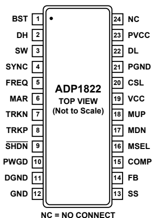
Figure 4. ADP1822 Pin Configuration
