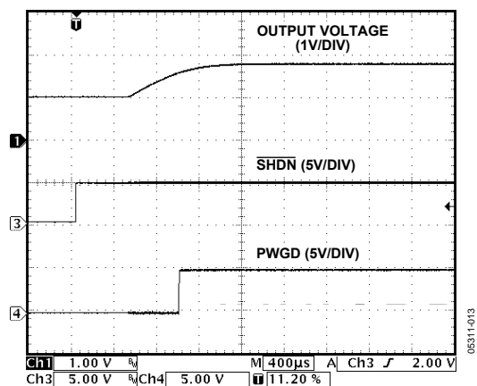
Figure 12. Power-On Response, Prebiased Output
