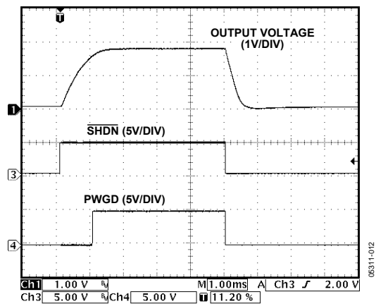
Figure 11. Power-On Response
