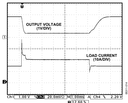
Figure 13. Output Short-Circuit Response and Recovery
