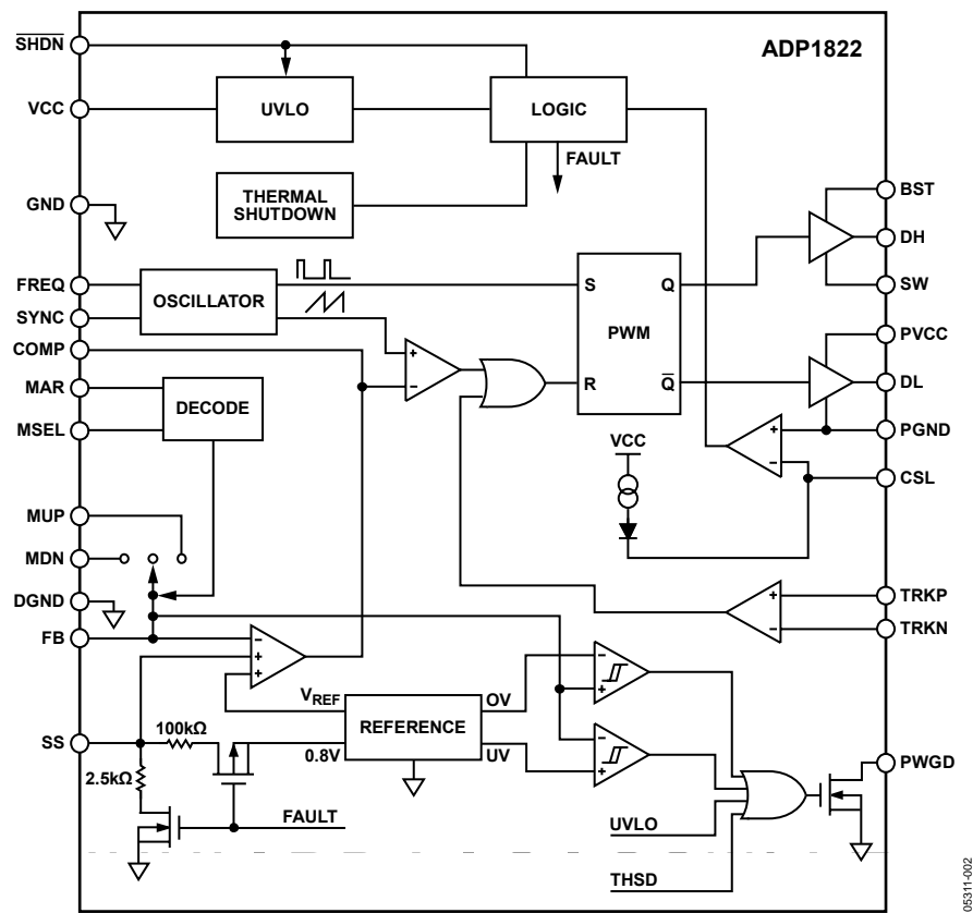
Figure 3. Simplified Block Diagram
