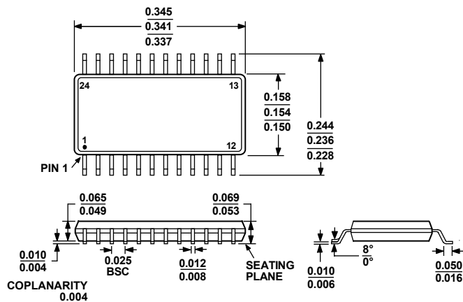
Figure 23. 24-Lead Shrink Small Outline Package [QSOP] (RQ-24) Dimensions shown in inches
