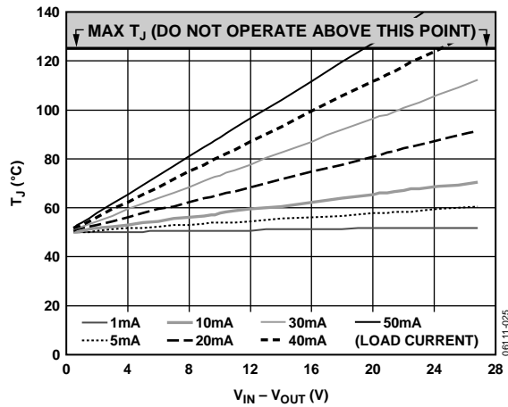
Figure 25. 300 mm² of PCB Copper, T_A = 50^\circ\text{C}
