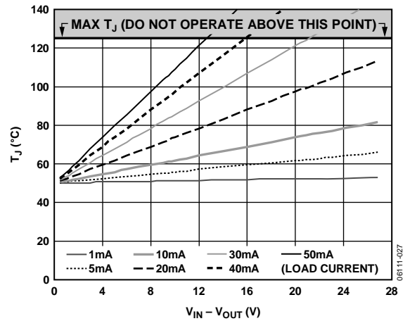
Figure 27. 0 mm² of PCB Copper, T_A = 50^\circ\text{C}
