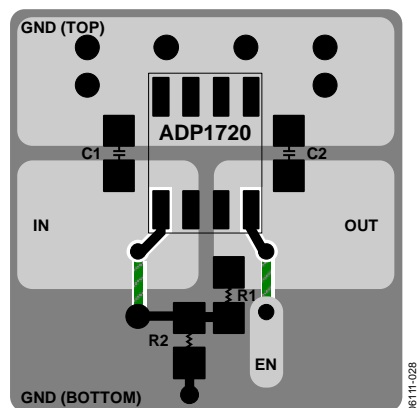
Figure 28. Example PCB Layout
