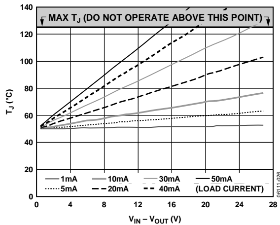
Figure 26. 100 mm² of PCB Copper, T_A = 50^\circ\text{C}
