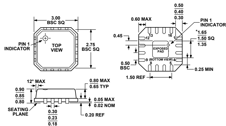
*COMPLIANT TO JEDEC STANDARDS MO-220-VEED-2 EXCEPT FOR EXPOSED PAD DIMENSION. Figure 36. 16-Lead Lead Frame Chip Scale Package [LFCSP_VQ] 3 mm x 3 mm Body, Very Thin Quad (CP-16-3) Dimensions shown in millimeters
