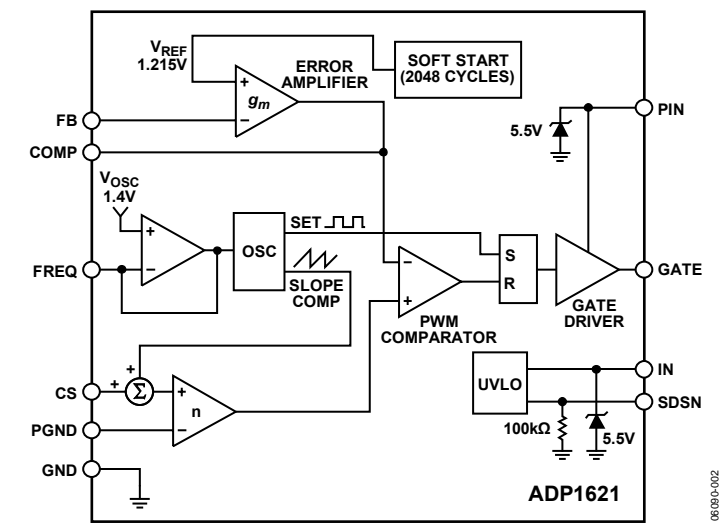
Figure 3. ADP1621 Simplified Block Diagram
