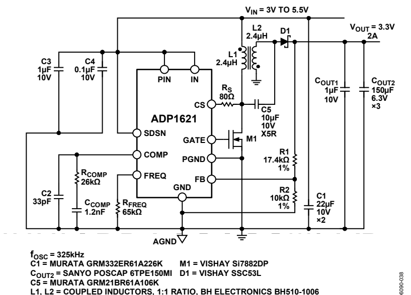
Figure 39. A SEPIC DC/DC Converter
