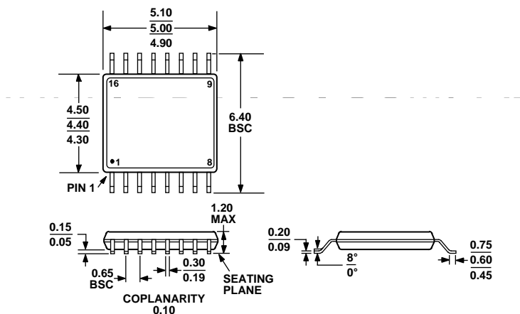
Figure 26. 16-Lead Thin Shrink Small Outline Package [TSSOP] (RU-16)
