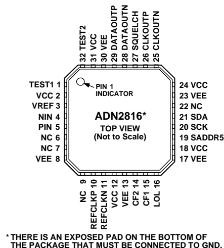
Figure 5. Pin Configuration
