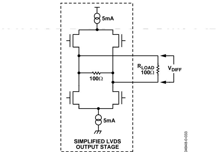
Figure 4. Differential Output Stage
