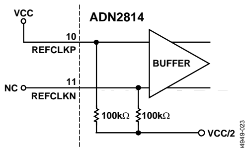
Figure 23. No REFCLK Configuration
