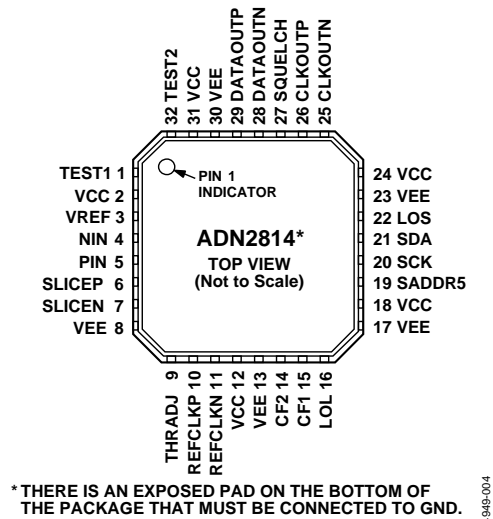
Figure 5. Pin Configuration
