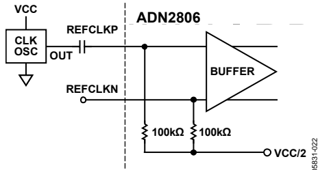
Figure 17. Single-Ended REFCLK Configuration
