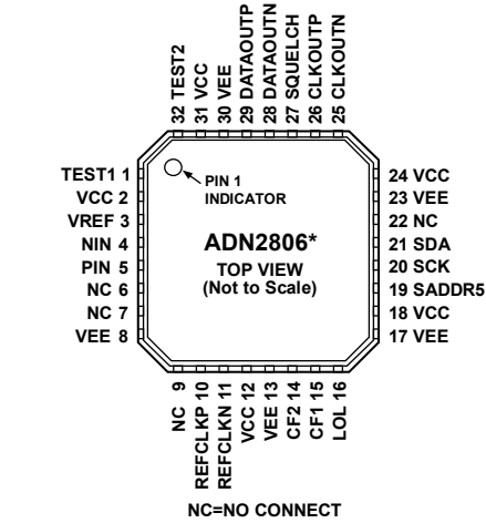
Figure 5. Pin Configuration
