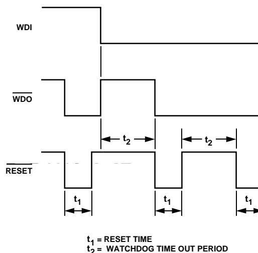
Figure 5. Watchdog Timeout Period and Reset Active Time
