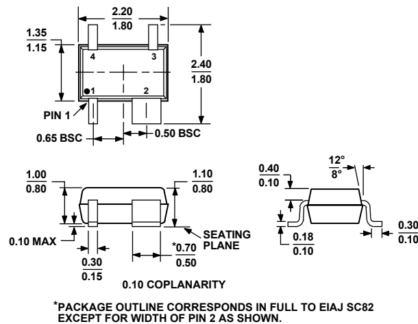
Figure 16. 4-Lead Thin Shrink Small Outline Transistor Package [SC70] (KS-4) Dimensions shown in millimeters
