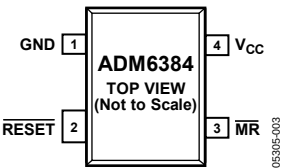
Figure 3. Pin Configuration
