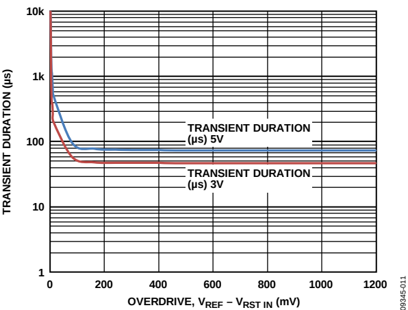
Figure 11. Maximum Transient Duration vs. RST IN ( V_{\text{TH}} = 1.23 \text{ V} ) Threshold Overdrive
