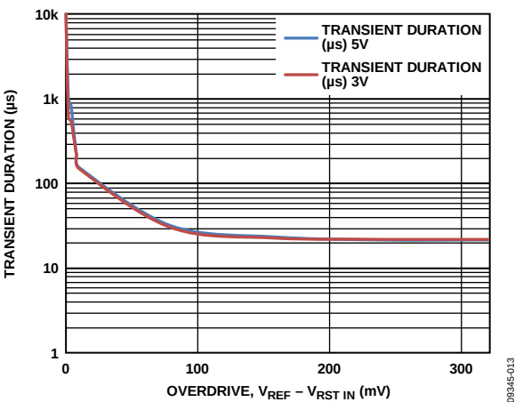
Figure 13. Maximum Transient Duration vs. RST INx ( V_{\text{TH}} = 0.4 \text{ V} ) Threshold Overdrive
