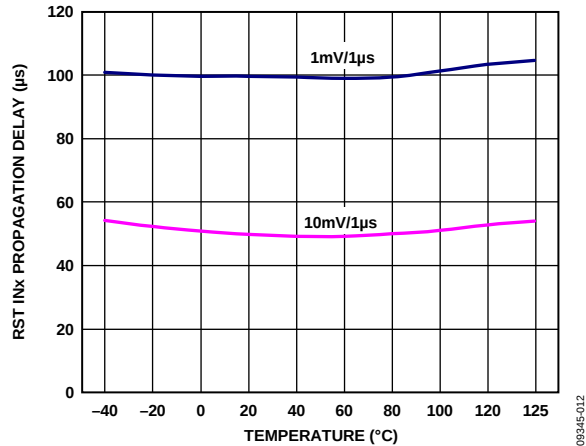
Figure 12. RST INx ( V_{\text{TH}} = 0.4 \text{ V} ) Falling Propagation Delay vs. Temperature
