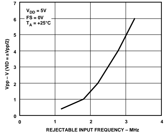
Figure 10. Rejectable Input Frequency vs. Amplitude
