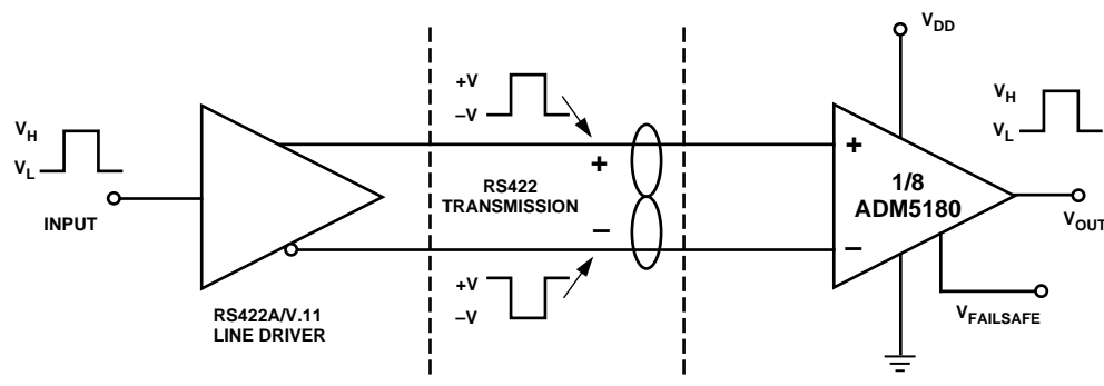
Figure 5. RS-422A/V.11 Data Transmission
