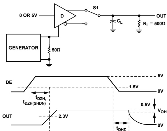
Figure 18. Driver Enable and Disable Times ( t_{DZH} , t_{DZL} , t_{DZH(SHDN)} )
