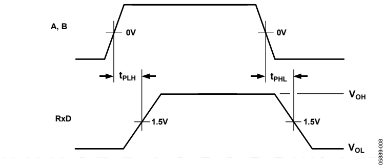
Figure 9. Receiver Propagation Delay
