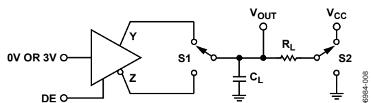
Figure 18. Driver Enable/Disable
