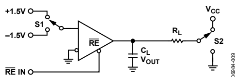
Figure 19. Receiver Enable/Disable
