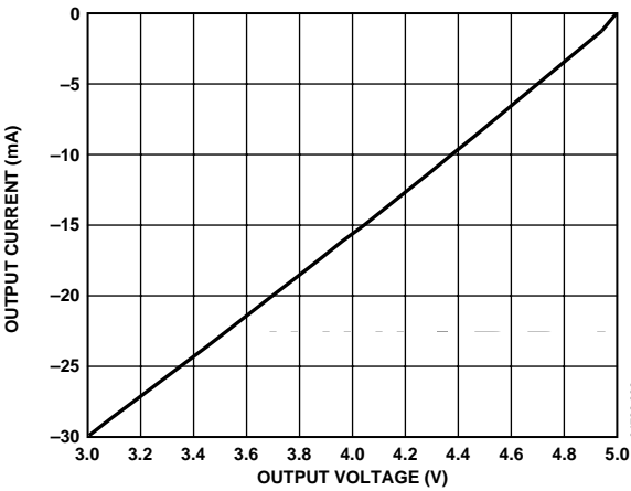
Figure 24. Output Current vs. Receiver Output High Voltage
