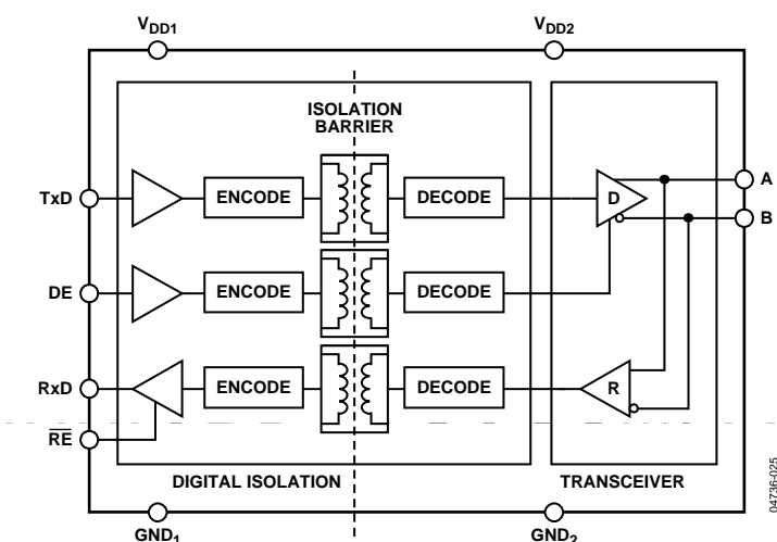
Figure 26. ADM2483 Digital Isolation and Transceiver Sections
