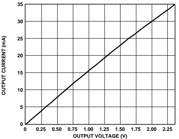
Figure 25. Output Current vs. Receiver Output Low Voltage
