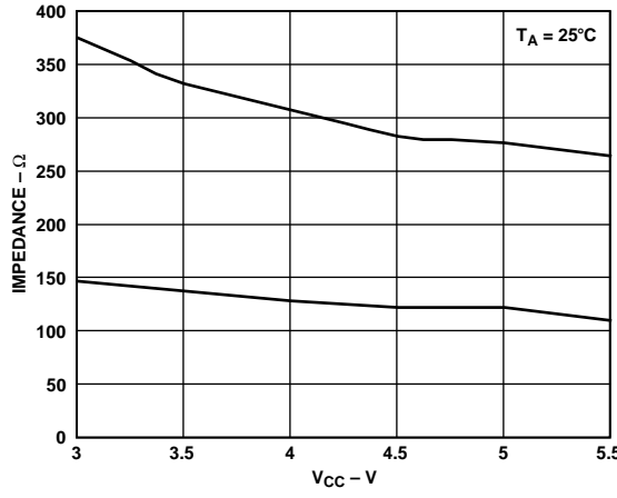
Figure 11. Charge Pump Impedance vs. V CC
