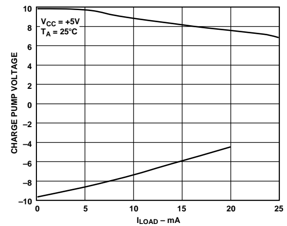
Figure 8. Charge Pump V + , V - vs. Current
