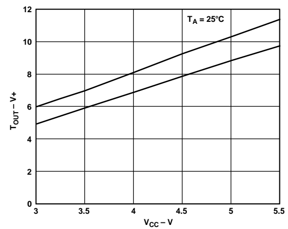
Figure 7. Transmitter Output Voltage High vs. V CC
