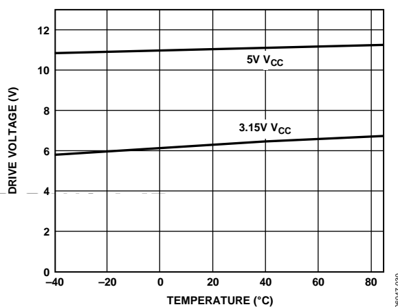
Figure 8. Drive Voltage ( V_{GATE} - V_{CC} ) vs. Temperature
