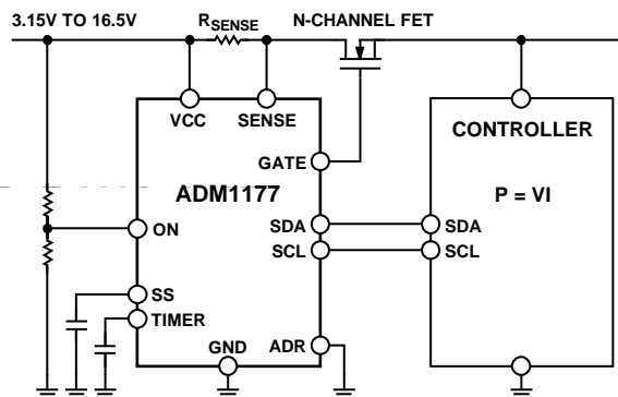
Figure 2. Applications Diagram
