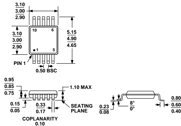
COMPLIANT TO JEDEC STANDARDS MO-187-BA Figure 47. 10-Lead Mini Small Outline Package [MSOP] (RM-10) Dimensions shown in millimeters
