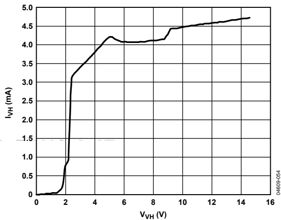
Figure 9. I_{VH} vs. V_{VH} ( V_{VH} as Supply)
