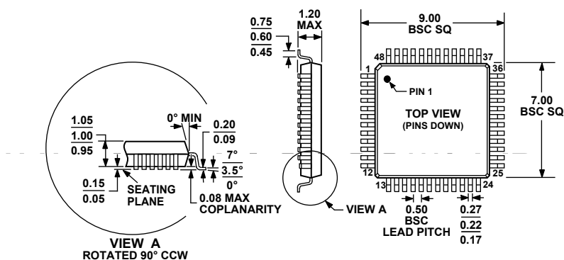
Figure 49. 48-Lead Thin Plastic Quad Flat Package [TQFP] (SU-48) Dimensions shown in millimeters
