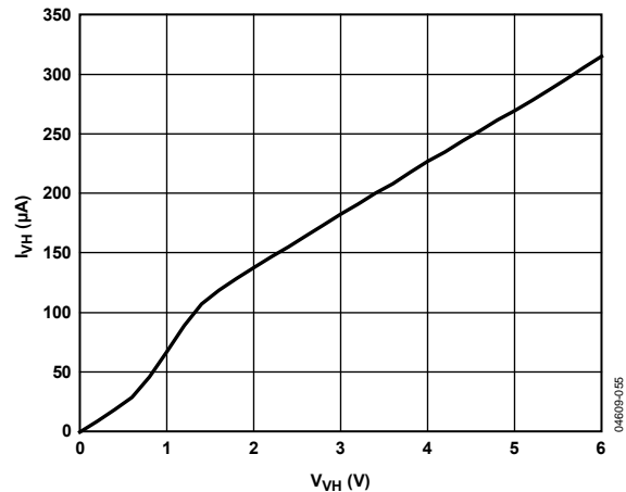
Figure 10. I_{VH} vs. V_{VH} ( V_{VH} Not as Supply)
