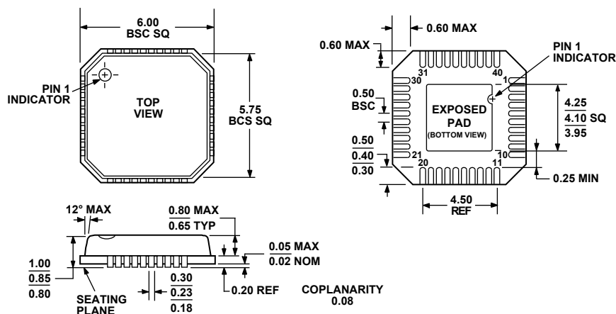
Figure 48. 40-Lead Lead Frame Chip Scale Package [LFCSP_VQ] 6 mm × 6 mm Body, Very Thin Quad (CP-40-1) Dimensions shown in millimeters
