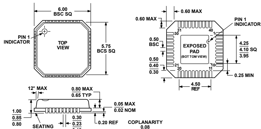
Figure 43. 40-Lead Lead Frame Chip Scale Package [LFCSP_VQ] 6 mm x 6 mm Body, Very Thin Quad (CP-40-1)
