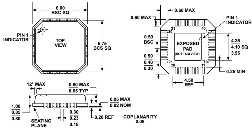
Figure 46. 40-Lead Lead Frame Chip Scale Package [LFCSP_VQ] 6 mm x 6 mm Body, Very Thin Quad (CP-40-1) Dimensions shown in millimeters
