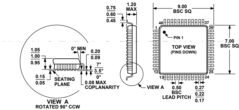
Figure 52. 48-Lead Thin Plastic Quad Flat Package [TQFP] (SU-48) Dimensions shown in millimeters
