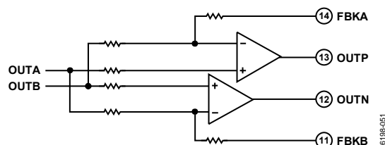
Figure 58. Op Amp Connections (All Resistors Are 1 k \Omega \pm 20%)
