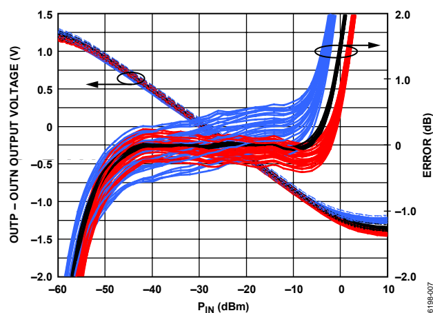
Figure 7. Distribution of [OUTP - OUTN] Gain Error and Voltage vs. Input Amplitude over Temperature, After Ambient Normalization for 45 Devices from a Nominal Lot, Frequency = 100 MHz, ADJA , ADJB = 0.65\text{ V} , 0.7\text{ V} , Sine Wave, Single-Ended Drive, P_{INH} = -30\text{ dBm} , Channel A Swept
