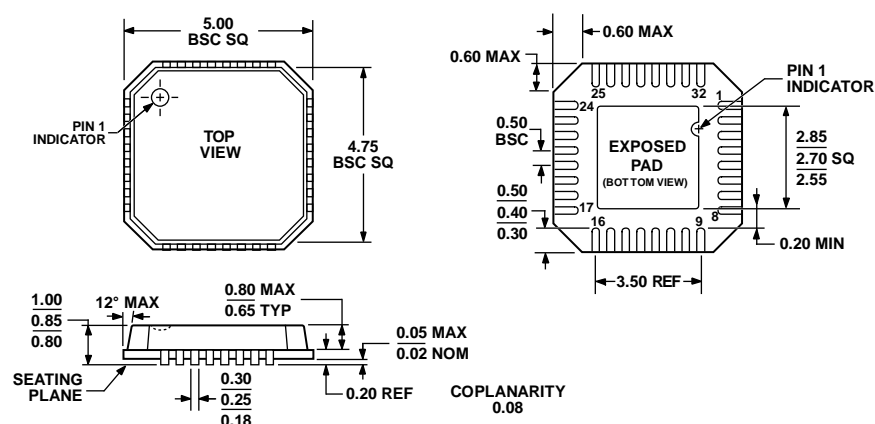
Figure 77. 32-Lead Lead Frame Chip Scale Package [LFCSP_VQ] 5 mm × 5 mm Body, Very Thin Quad Lead (CP-32-8) Dimensions shown in millimeters
