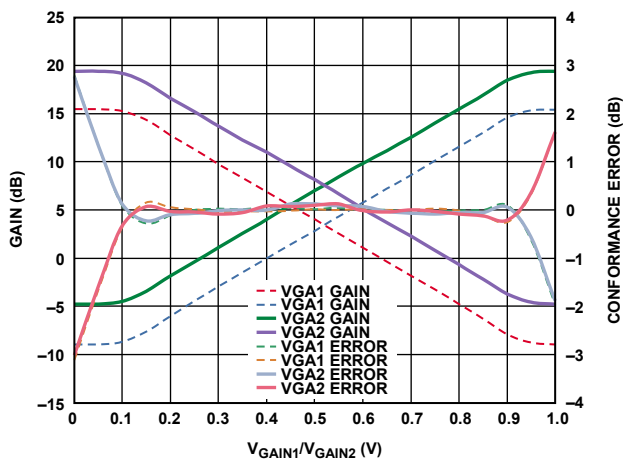
Figure 61. Gain and Conformance Error vs. V_{\text{GAIN1}}/V_{\text{GAIN2}} for Gain Code 11, and \text{MODE} = 0 \text{ V} and \text{MODE} = 5 \text{ V} for Both VGAs
