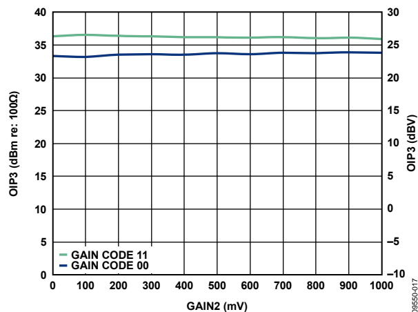
Figure 15. OIP3 vs. V_{\text{GAIN}} over Gain Code for VGA2
