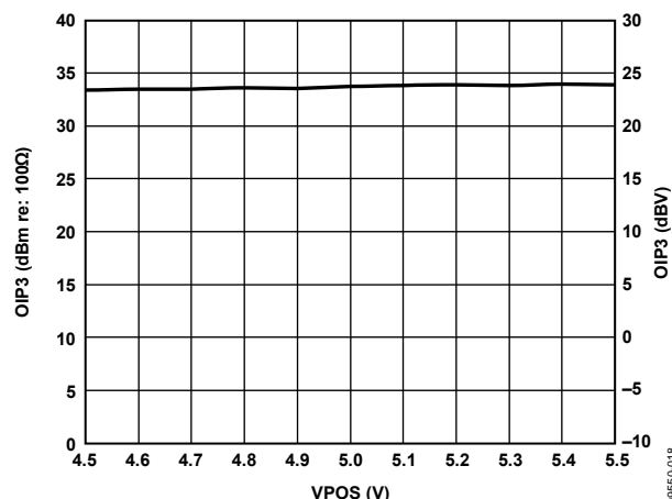
Figure 16. OIP3 vs. Supply Voltage at V_{\text{GAIN}} = 0.5 V for VGA2
