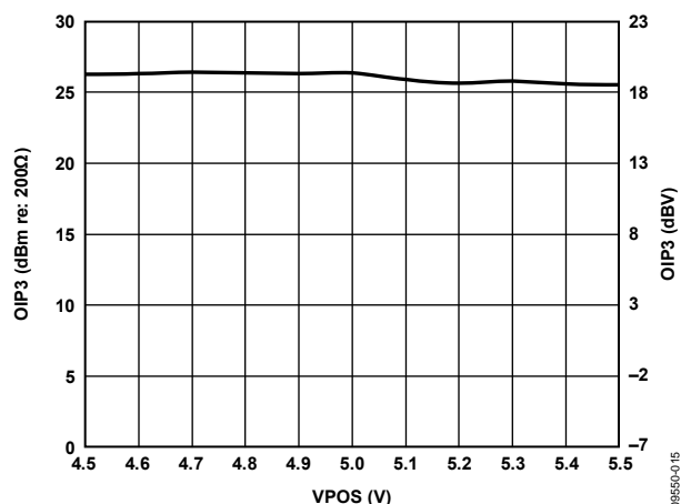
Figure 13. OIP3 vs. Supply Voltage at V_{\text{GAIN}} = 0.5 V for VGA1
