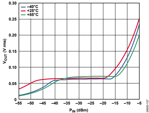
Figure 53. V_{OUT} vs. Input Power ( P_{IN} ) over temperature for VGA1
