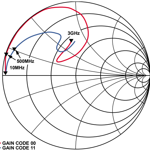
Figure 41. S_{22} (re: 50\ \Omega ) vs. V_{GAIN} over Gain Code for VGA1
