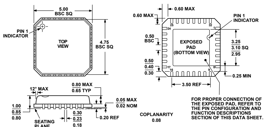
Figure 74. 32-Lead Lead Frame Chip Scale Package [LFCSP_VQ] 5 mm × 5 mm Body, Very Thin Quad (CP-32-2) Dimensions shown in millimeters
