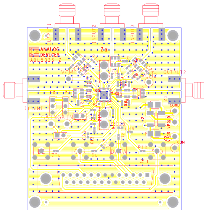
Figure 71. Silkscreen Top
