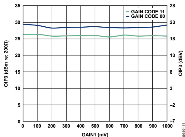
Figure 12. OIP3 vs. V_{\text{GAIN}} over Gain Code for VGA1
