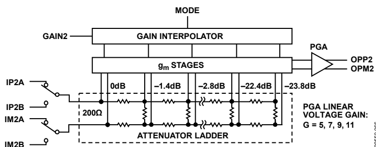
Figure 60. VGA2 Functional Block Diagram
