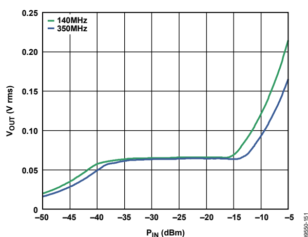
Figure 51. V_{OUT} vs. Input Power ( P_{IN} ) over Frequency (AGC Mode) for VGA2
