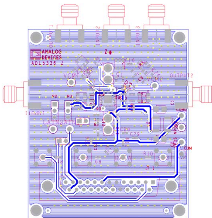
Figure 72. Silkscreen Bottom
