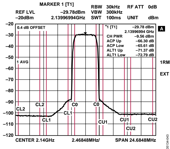
Figure 43. Single-Carrier WCDMA Spectrum at 2140 MHz; V_{\text{GAIN}} = 1.4 \text{ V} , P_{\text{IN}} = -23 \text{ dBm}
