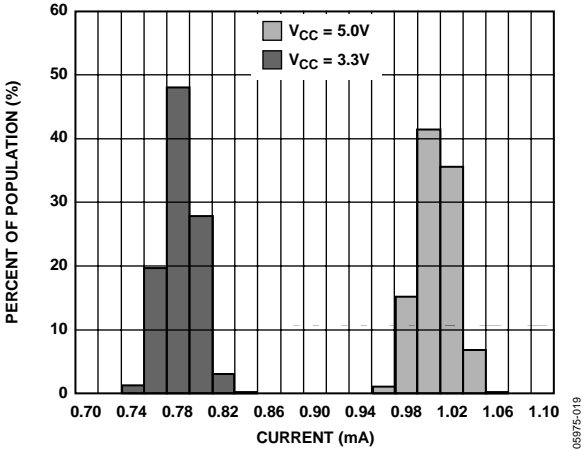
Figure 20. Power-Down Supply Current
