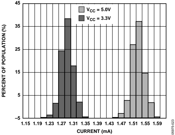
Figure 19. Supply Current at 25°C
