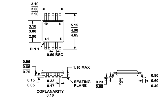
COMPLIANT TO JEDEC STANDARDS MO-187-BA Figure 29. 10-Lead Mini Small Outline Package [MSOP] (RM-10) Dimensions shown in millimeters
