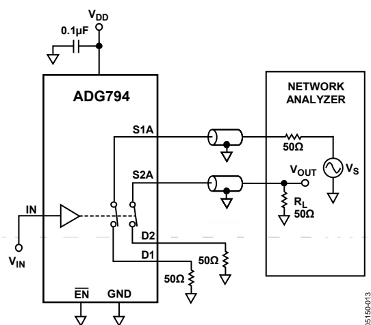
Figure 15. Channel-to-Channel Crosstalk
