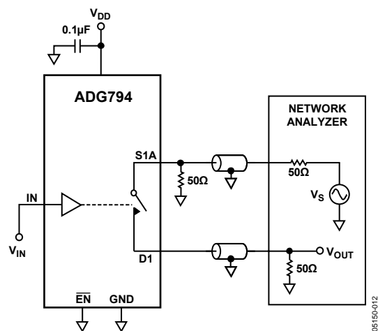
Figure 14. Off Isolation
