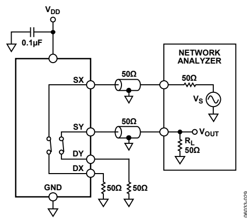
Figure 27. Channel-to-Channel Crosstalk
