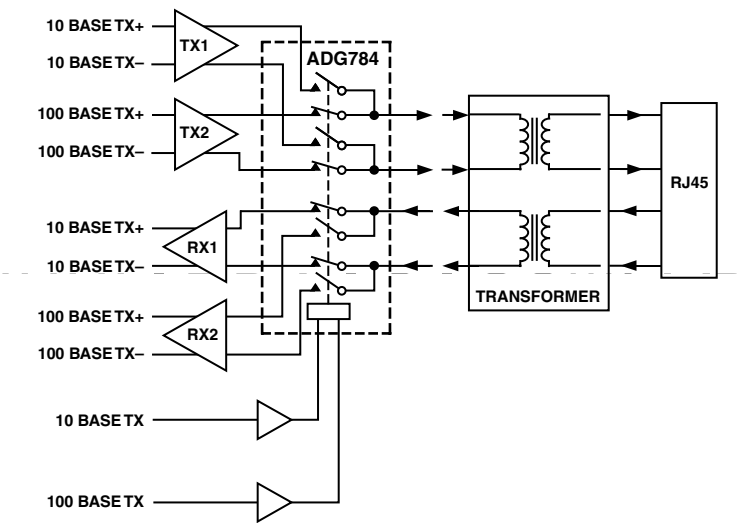
Figure 1. Full Duplex Transceiver
