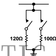
Figure 27. Line Termination
