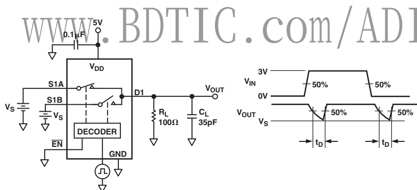
Test Circuit 5. Break-Before-Make Time Delay
