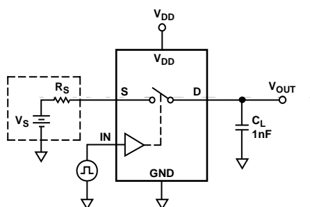
Figure 15. Charge Injection
