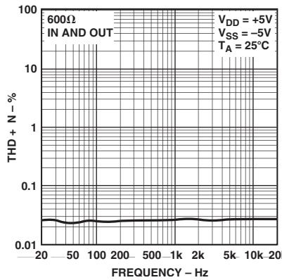
TPC 14. THD + Noise
