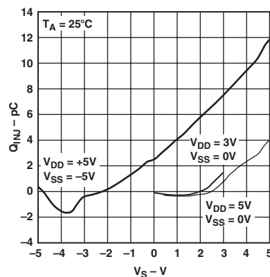
TPC 8. Charge Injection vs. Source Voltage
