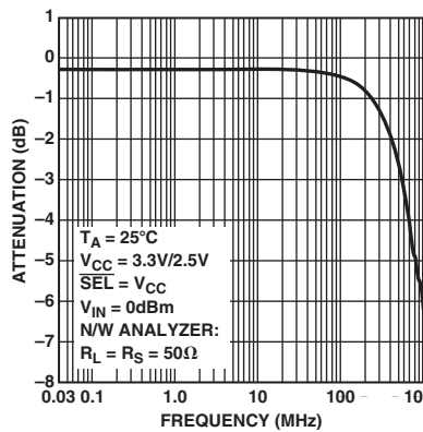
TPC 13. Bandwidth vs. Frequency
